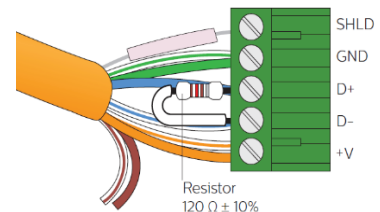
E12 Range, Resistor 120Ω, 10% Tolerance, Carbon Film
