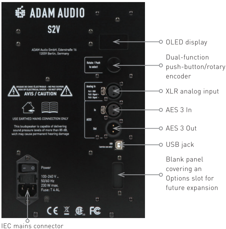
IEC mains connector
